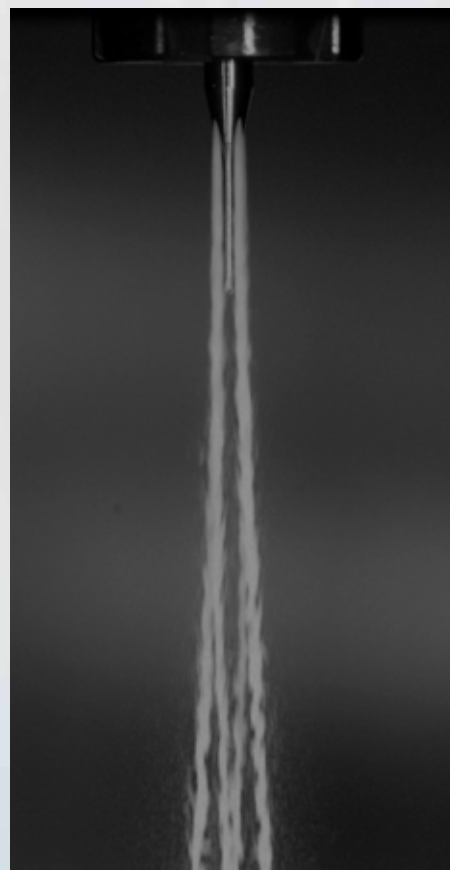
Internal cooling with 80 bar with S=24,000 rev./min
