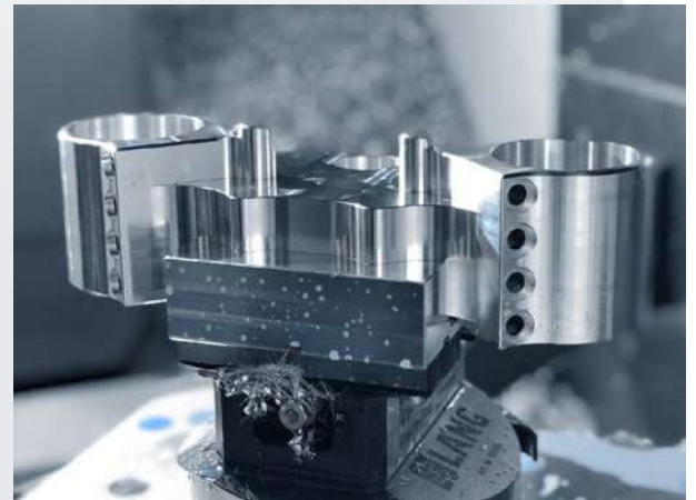
Profilo 77 Profile Clamping Vice
