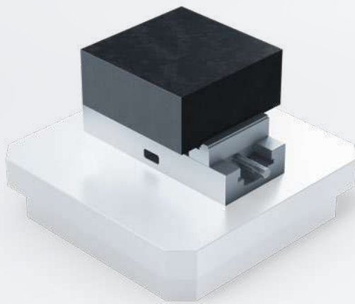
Conventional vice on automation pallet 400 × 400 mm. Workpiece dimensions 205 × 205 × 90 mm.
