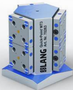
Quick-Point® 3-Face & 4-Face Tombstone
